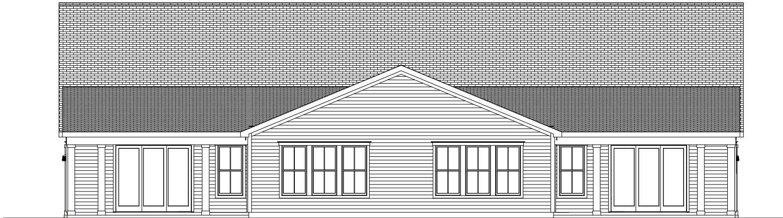
Duplex A Rear Elevation
